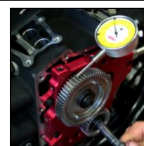
Measuring Back Lash
